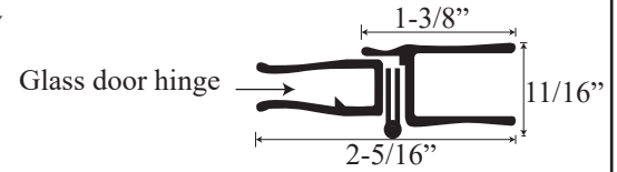
Section or Side view
