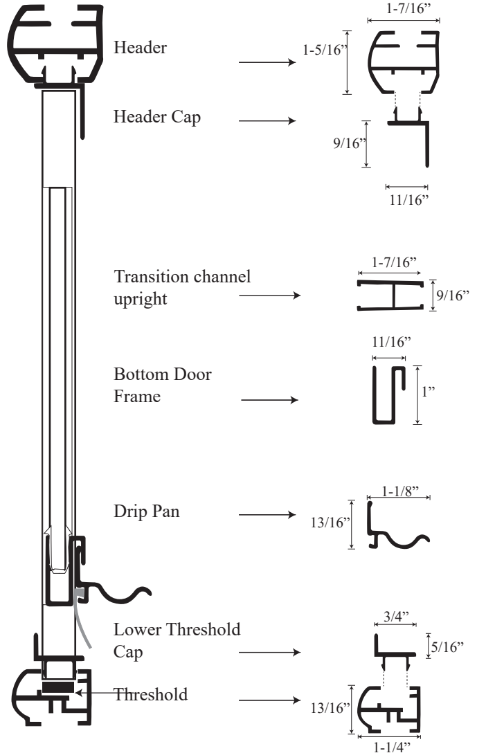
Section or Side view
