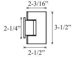
Wall Mount Hinge →
