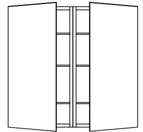
Left and Right Hand Cabinets with Connection Kit
